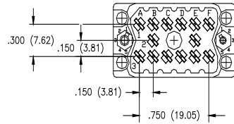
14 PIN PLUG
