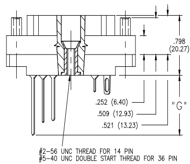
RECEPTACLE WITH LOCKNUT AND POLARIZING SOCKETS
