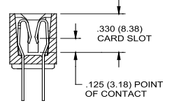
INSULATOR STYLE CODE 5
