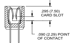
INSULATOR STYLE CODE 2
